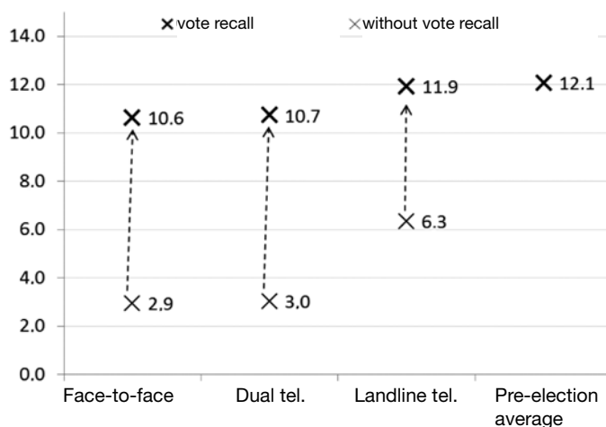
FIGURE 6. Absolute error
